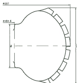
CROSS SECTION OF MOUNTED TIRE
