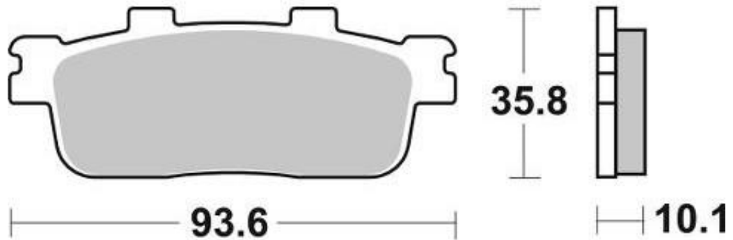
SBS 201MS / WG-7447F8 / WG-8201F8
