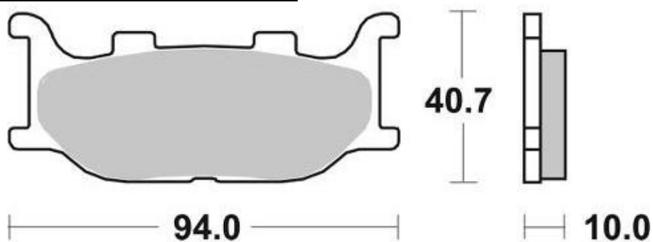
SBS 128MS / WG-7291F8 / WG-8147F8
